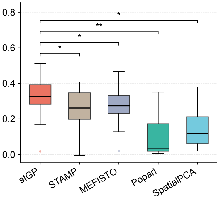
ARI
